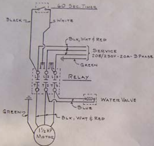
THREE PHASE
